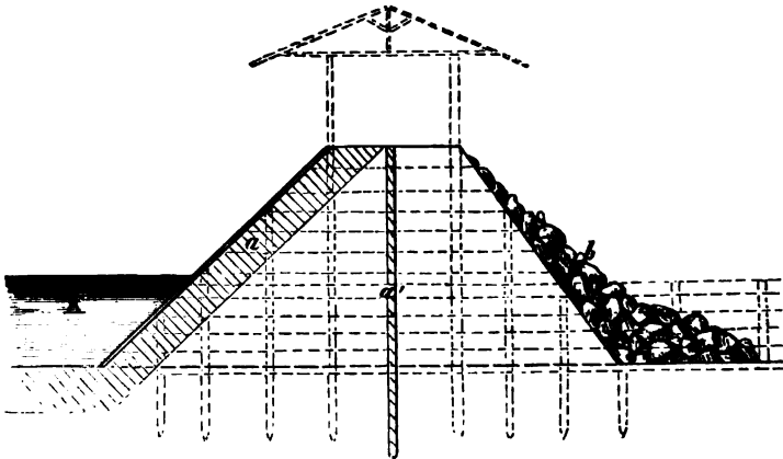
Fig. 230.—Earth-dam.
